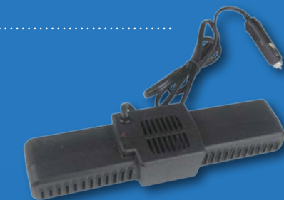
WS06007 DC12V Car heater • Specification:Max wind speed:0.3M/S;Max • wind temperature:45℃ • Winter necessity for car.
